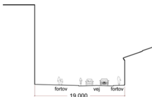
Snit F-F
